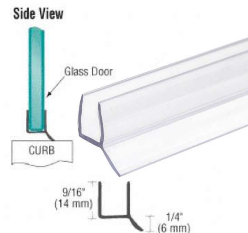
PART PVC-14SL-3/8
