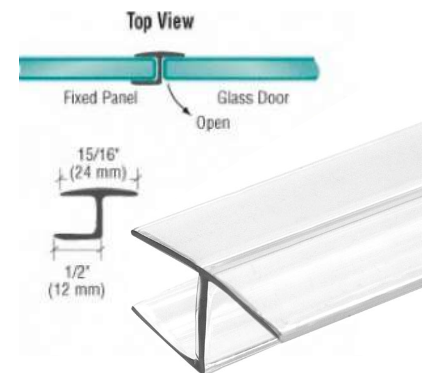
PVC-26-1/2
